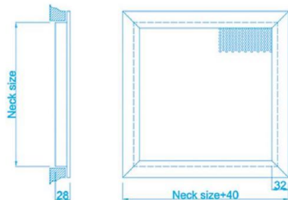
Perforated Flat Diffuser
